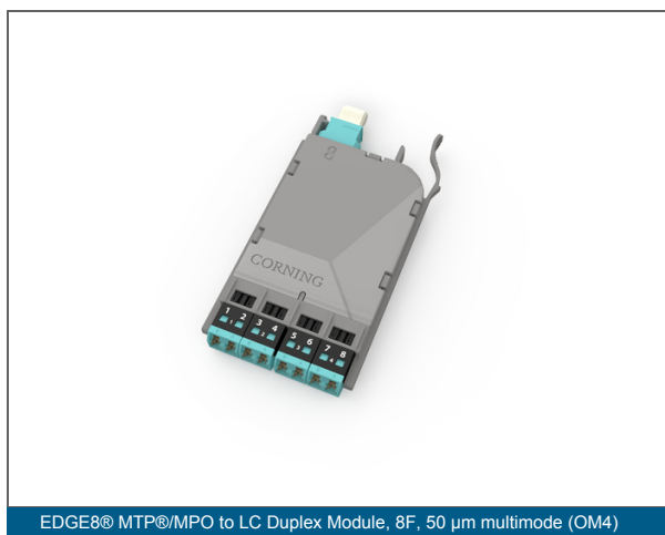
EDGE8® MTP®/MPO to LC Duplex Module, 8F, 50 µm multimode (OM4)
