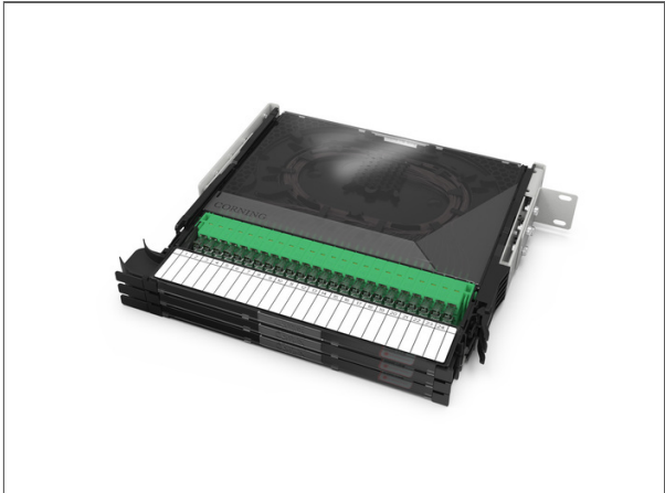
Centrix™ loaded housing, 1U, 3 cassettes, 24xSC/APC adapters + SF pigtails, 72 ports, HS
