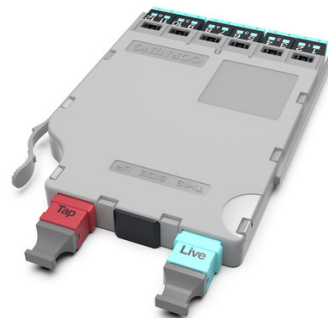
EDGE™ Solutions Tap Module, 50 µm MM (OM4), 50/50 split ratio (live/tap), 12F LC duplex ports, one pinned MTP® adapter labeled LIVE, one pinned red MTP adapter labeled TAP, enables six monitored ports, Universal Polarity
