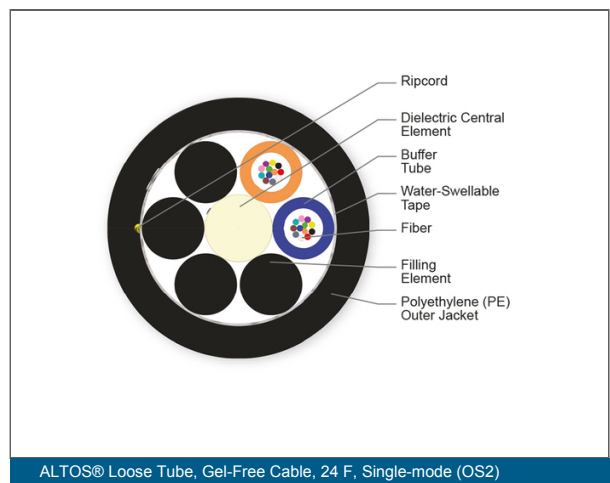
ALTOS® Loose Tube, Gel-Free Cable, 24 F, Single-mode (OS2)
