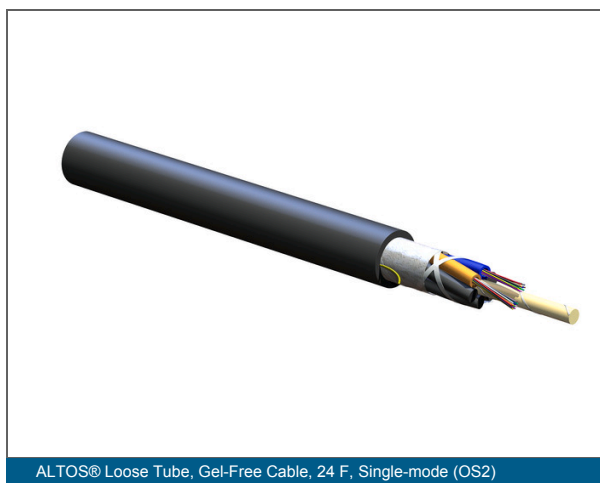
ALTOS® Loose Tube, Gel-Free Cable, 24 F, Single-mode (OS2)
