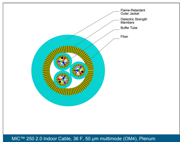
MIC™ 250 2.0 Indoor Cable, 36 F, 50 µm multimode (OM4), Plenum
