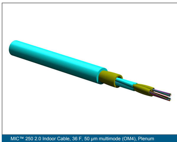
MIC™ 250 2.0 Indoor Cable, 36 F, 50 µm multimode (OM4), Plenum
