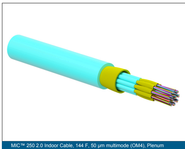
MIC™ 250 2.0 Indoor Cable, 144 F, 50 µm multimode (OM4), Plenum
