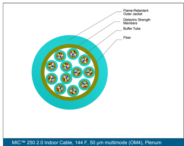
MIC™ 250 2.0 Indoor Cable, 144 F, 50 µm multimode (OM4), Plenum
