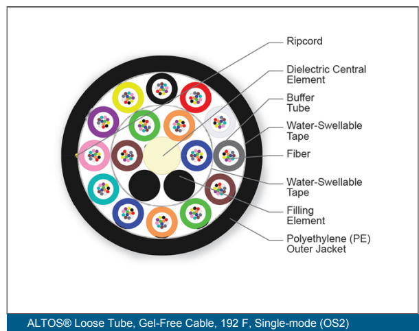
ALTOS® Loose Tube, Gel-Free Cable, 192 F, Single-mode (OS2)
