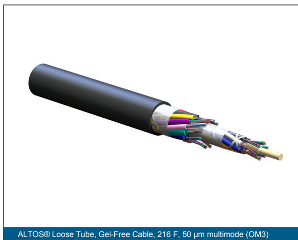
ALTOS® Loose Tube, Gel-Free Cable, 216 F, 50 \mu m multimode (OM3)
