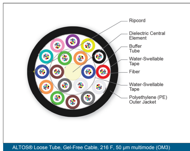
ALTOS® Loose Tube, Gel-Free Cable, 216 F, 50 \mu m multimode (OM3)
