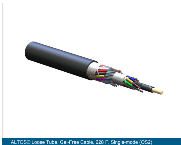
ALTOS® Loose Tube, Gel-Free Cable, 228 F, Single-mode (OS2)
