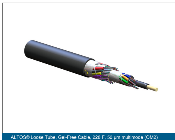
ALTOS® Loose Tube, Gel-Free Cable, 228 F, 50 µm multimode (OM2)
