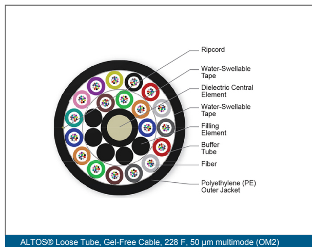
ALTOS® Loose Tube, Gel-Free Cable, 228 F, 50 µm multimode (OM2)
