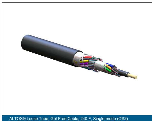
ALTOS® Loose Tube, Gel-Free Cable, 240 F, Single-mode (OS2)
