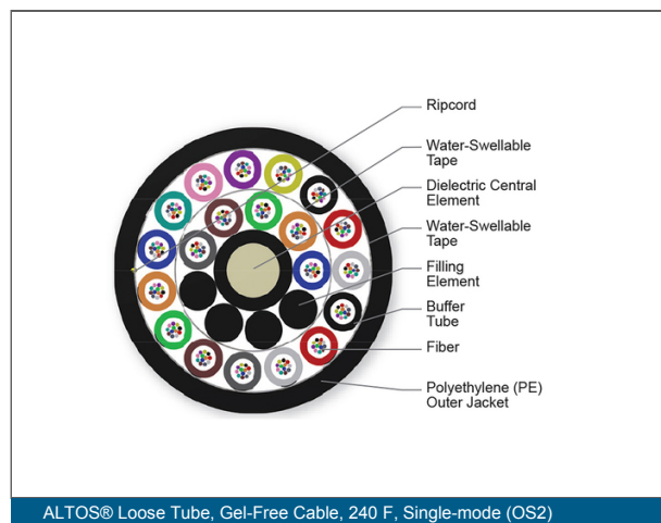
ALTOS® Loose Tube, Gel-Free Cable, 240 F, Single-mode (OS2)
