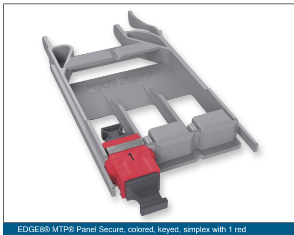
EDGE8® MTP® Panel Secure, colored, keyed, simplex with 1 red
