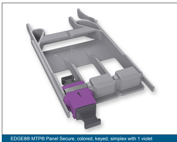
EDGE8® MTP® Panel Secure, colored, keyed, simplex with 1 violet
