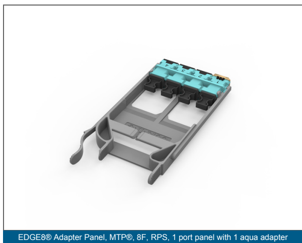
EDGE8® Adapter Panel, MTP®, 8F, RPS, 1 port panel with 1 aqua adapter
