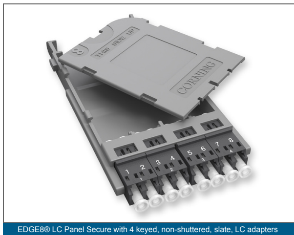
EDGE8® LC Panel Secure with 4 keyed, non-shuttered, slate, LC adapters
