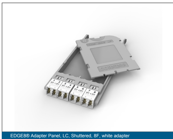
EDGE8® Adapter Panel, LC, Shuttered, 8F, white adapter
