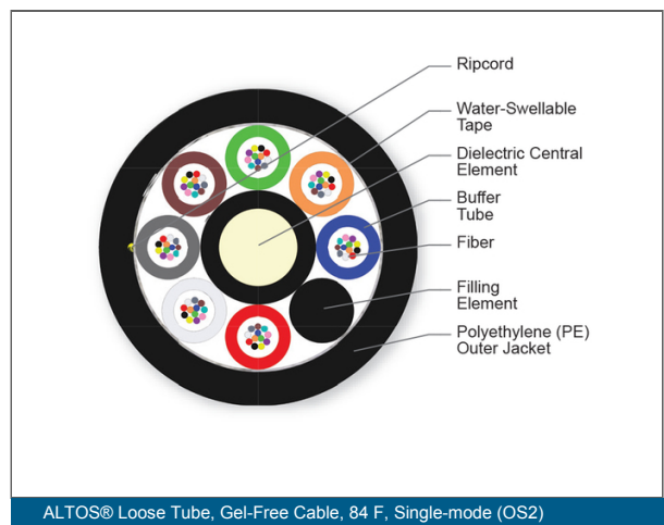
ALTOS® Loose Tube, Gel-Free Cable, 84 F, Single-mode (OS2)
