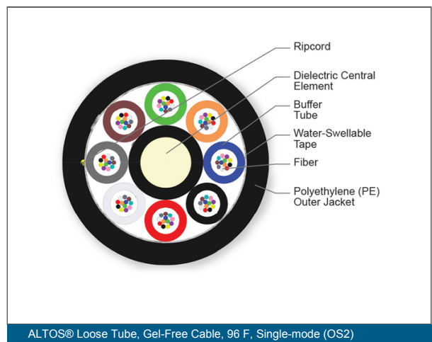
ALTOS® Loose Tube, Gel-Free Cable, 96 F, Single-mode (OS2)
